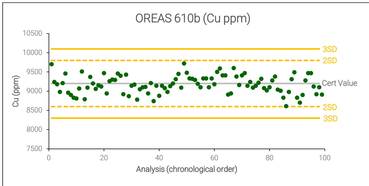
Figure 11.13 2024-2025 OREAS 610b Copper Assay Results
