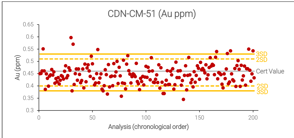
Figure 11.5 2024-2025 CDN-CM-51 Gold Assay Results
