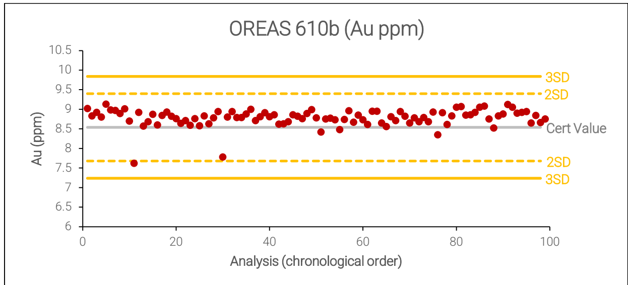
Figure 11.7 2024-2025 OREAS 610b Gold Assay Results
