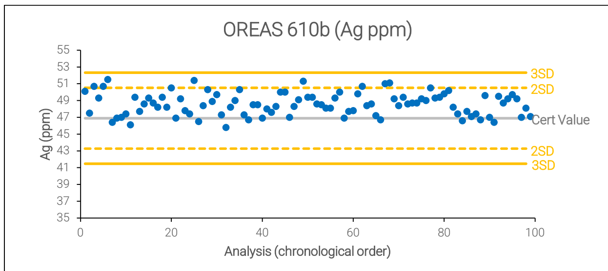
Figure 11.10 2024-2025 OREAS 610b Silver Assay Results
