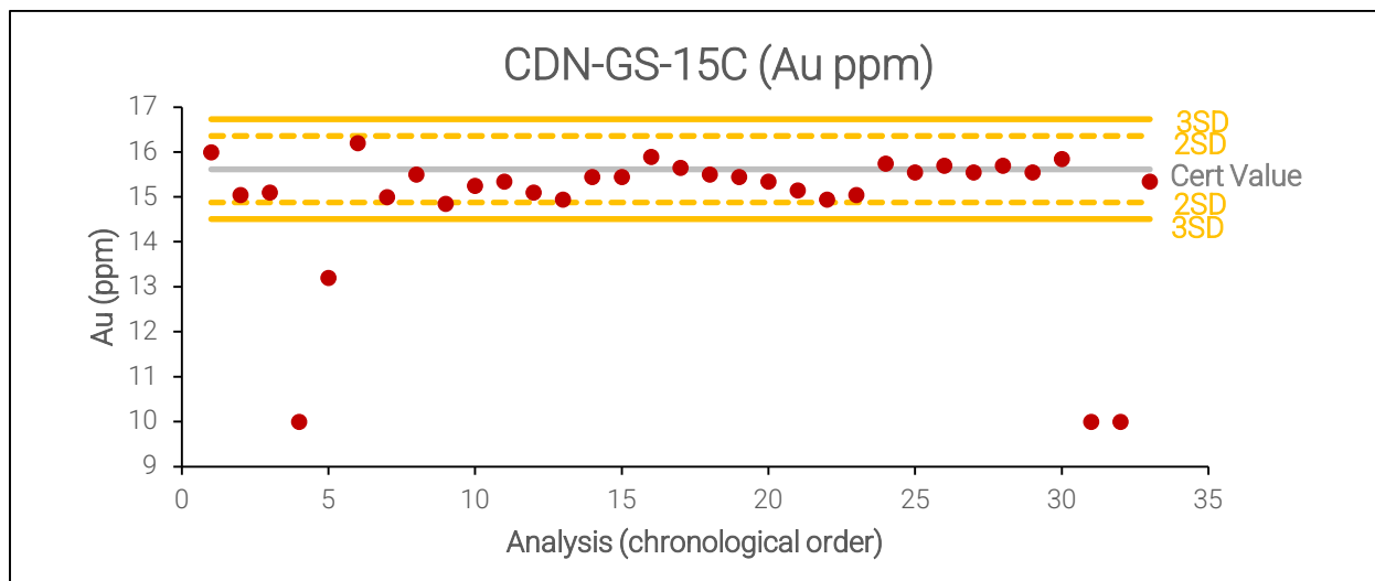
Figure 11.8 2024-2025 CDN-GS-15C Gold Assay Results
