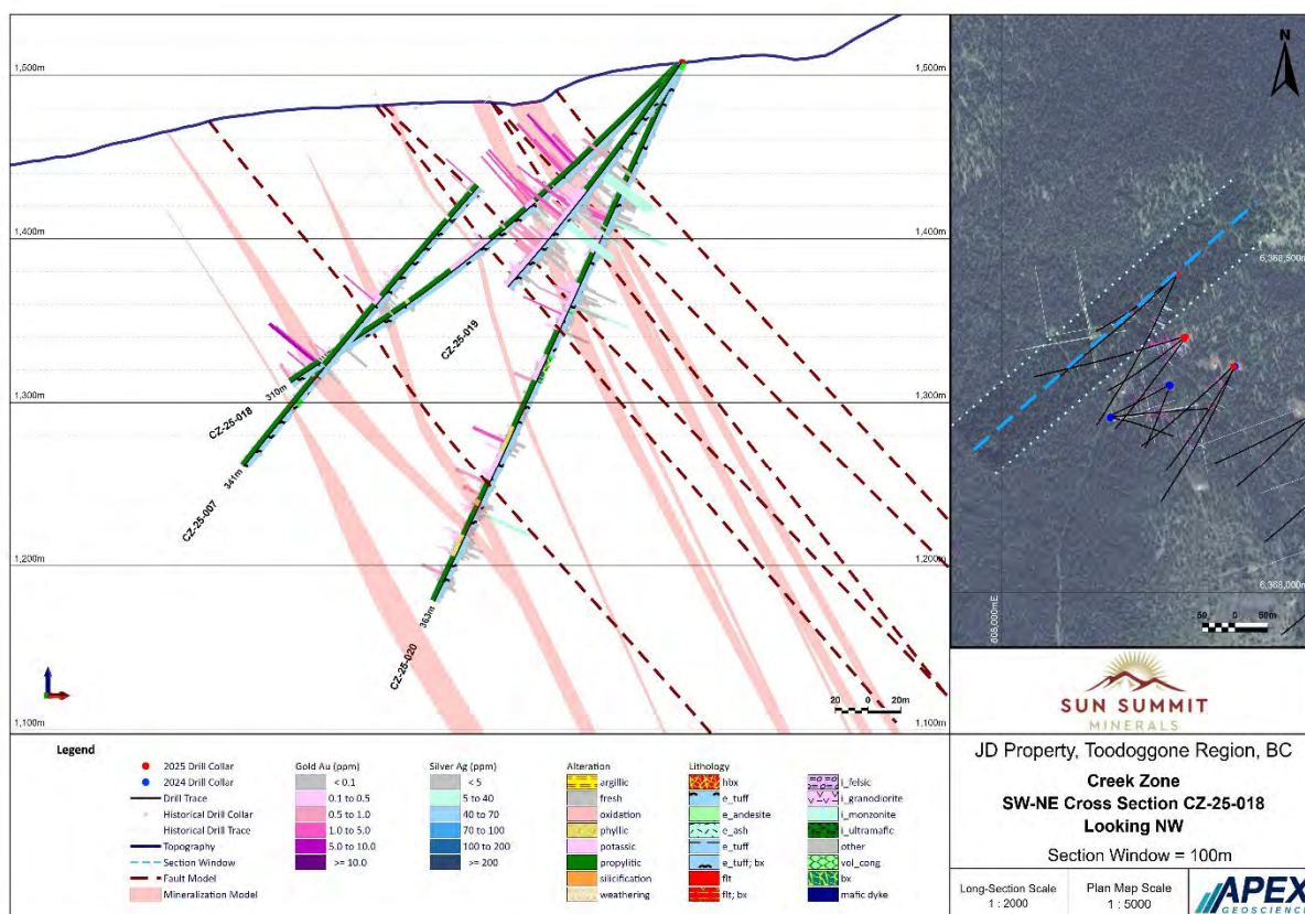
Figure 10.7 Cross Section Creek zone CZ-25-018 looking NW
