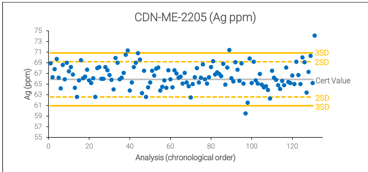
Figure 11.9 2024-2025 CDN-ME-2205 Silver Assay Results
