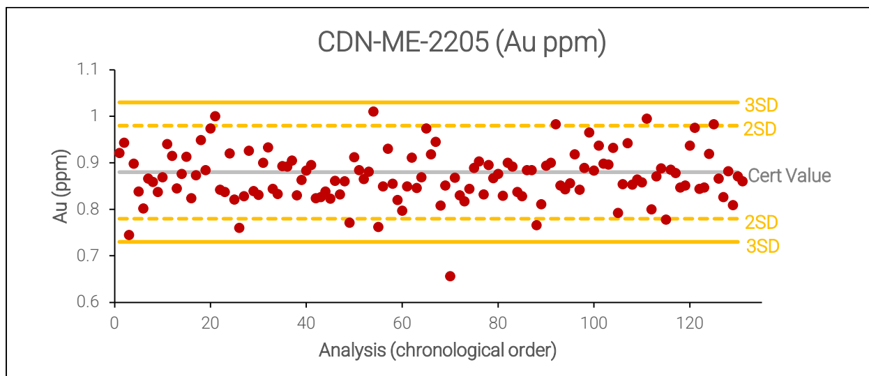
Figure 11.6 2024-2025 CDN-ME-2205 Gold Assay Results
