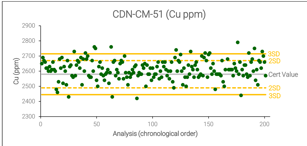
Figure 11.11 2024-2025 CDN-CM-51 Copper Assay Results
