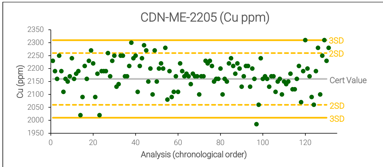
Figure 11.12 2024-2025 CDN-ME-2205 Copper Assay Results
