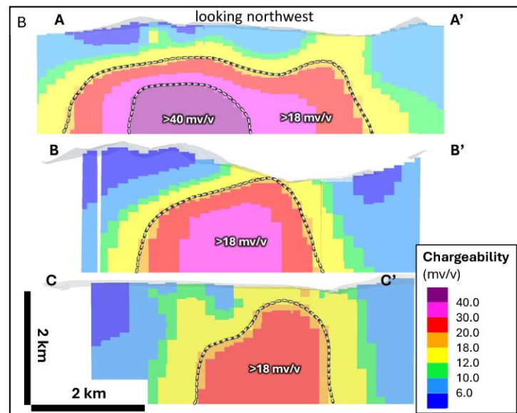
(B) Sections through the chargeability 3D voxel model showing the strong-chargeability anomaly at Fericrete (A-A'), McClair (B-B') and Belle South (C-C') targets. Section lines shown in (A).
