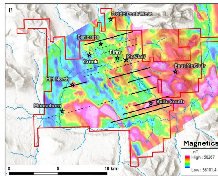
(B) Map of the JD Project showing total magnetic intensity data acquired in 2021 overlain with IP lines and key target areas.
