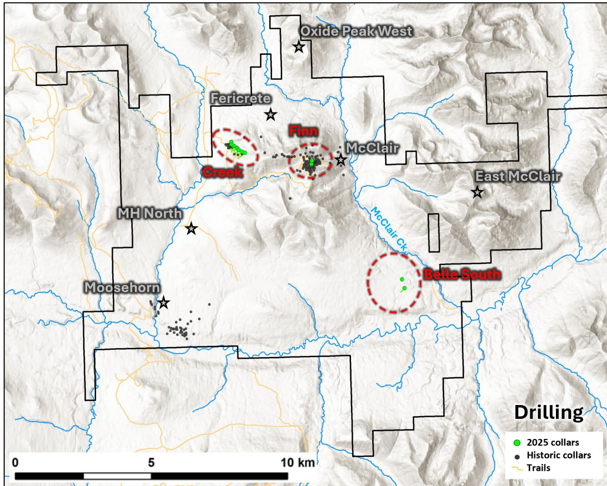
Figure 2. Map of JD Project showing the locations of all 2025 drill collars and the locations of all historic drill collars. Targets circled in red (Creek, Finn, and Belle South) were the focus of 2025 drilling. The targets with grey stars were advanced in 2025 through programs consisting of varying proportions of mapping, geochemistry, and geophysics.
