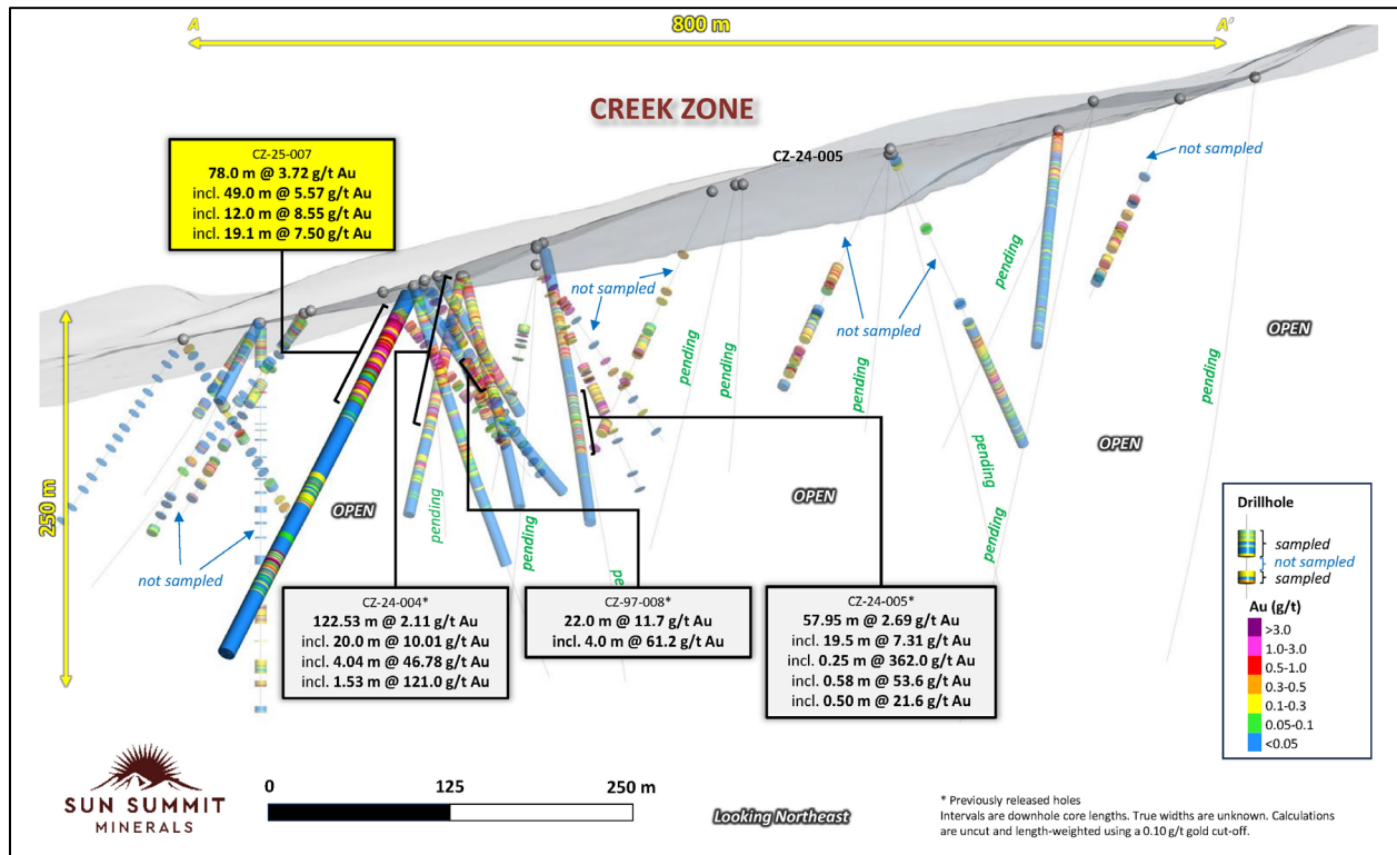
Figure 1. Oblique view through the Creek Zone drill holes showing downhole assays for all drill holes including CZ-25-007 and holes with pending results. Selected highlights from the 2024 drill program at the Creek Zone are also shown (see news releases of Sun Summit dated (i) October 2, 2024 and entitled "Sun Summit Drills 122.5 m of 2.1 g/t Gold Including 20.0 m of 10.0 g/t Gold at the Creek Zone, JD Project, Toodoggone District, B.C.", and (ii) October 16, 2024 and entitled "Sun Summit drills 57.95 m of 2.69 g/t gold including 19.50 m of 7.31 g/t gold at the Creek Zone, JD Project, Toodoggone District, B.C."). See references 1 and 2 for sources of historical drill data.
